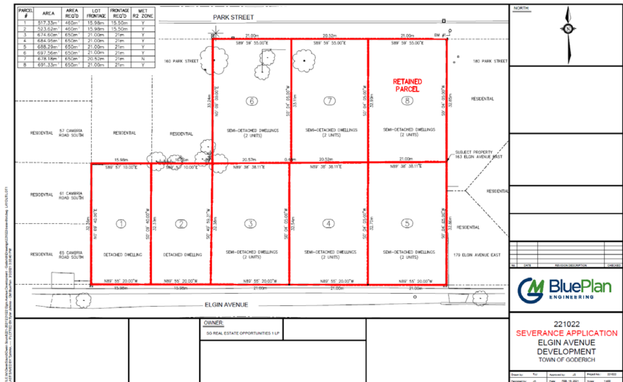
Figure 1. Severance Sketch, provided by GM BluePlan Engineering
