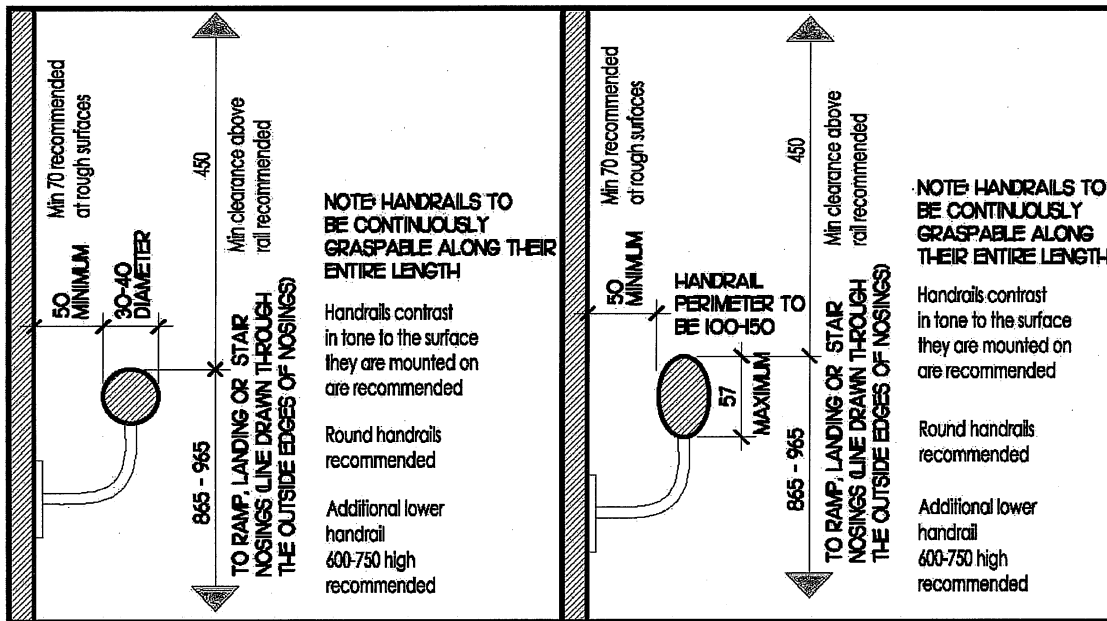
Figure 1.6 Handrail Dimensions (Global Alliance on Accessible Technologies and Environments, 2014)
