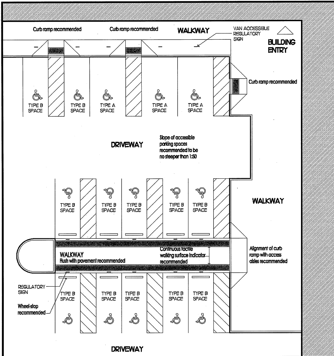
Figure 1.15 Design Criteria for Access Aisles (Global Alliance on Accessible Technologies and Environments, 2014)
